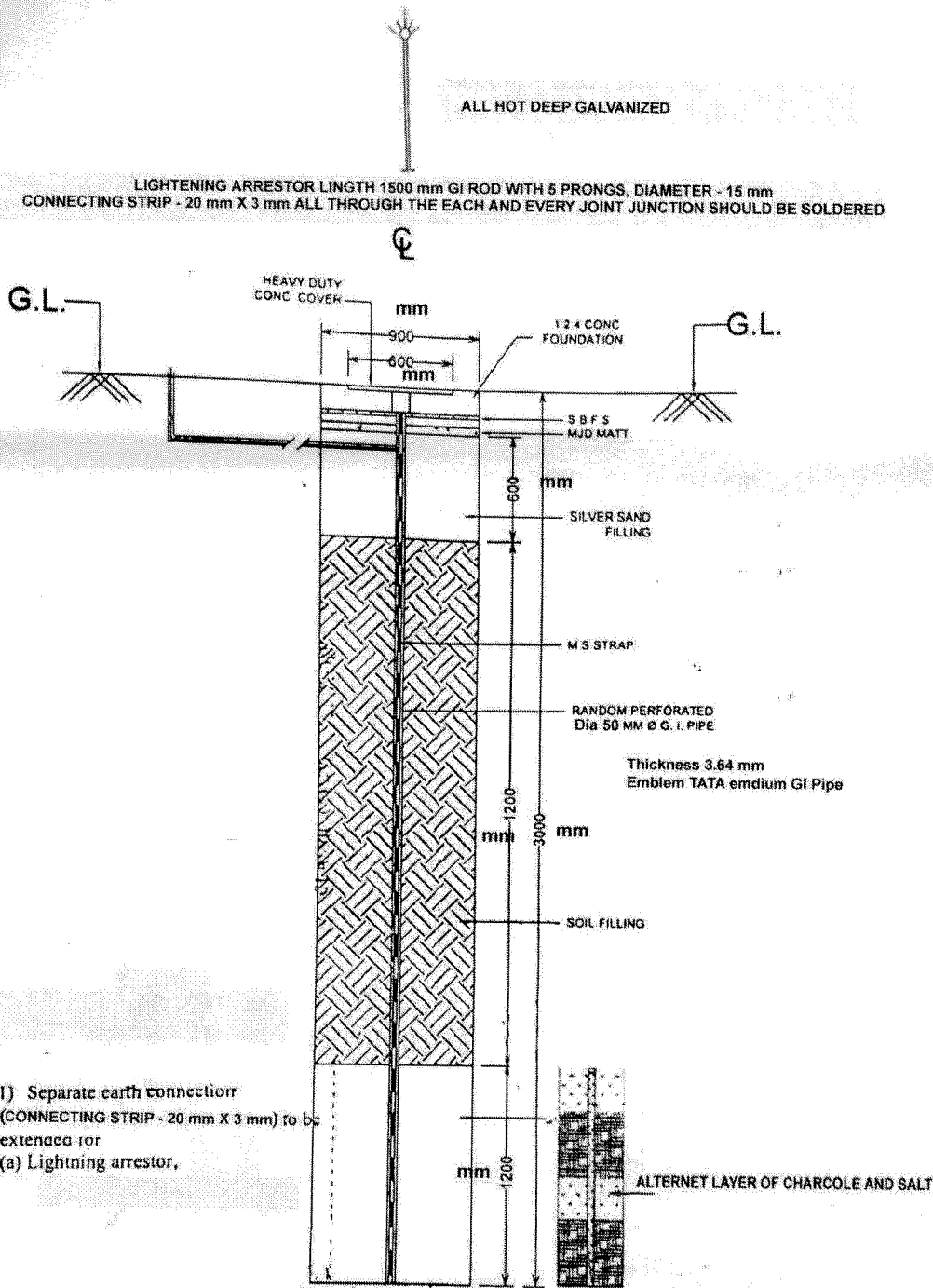
DETAIL OF TYPICAL LIGHTENING ARRESTOR WITH EARTHING
