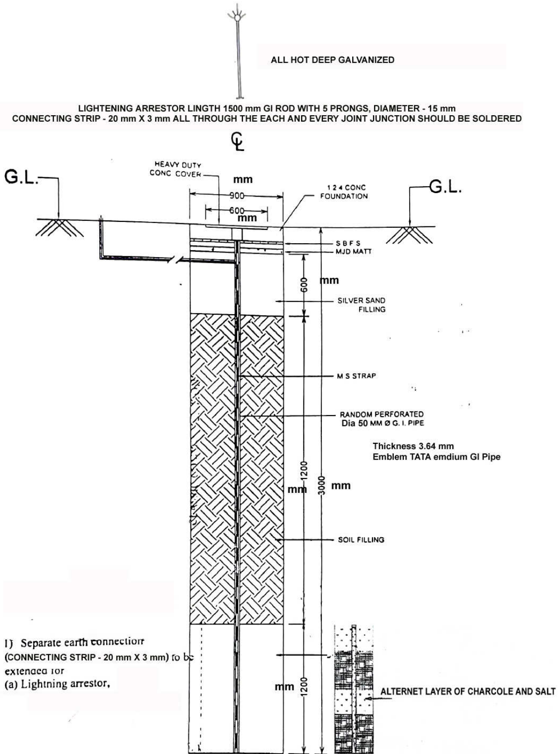
DETAIL OF TYPICAL LIGHTNING ARRESTOR WITH EARTHING
